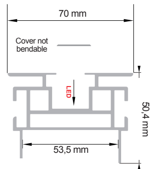
ARCS 16 with LEDs
