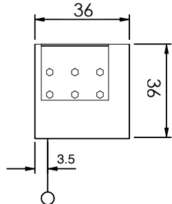
36x36 casing profile between 7m and 8m base Power supply on the right
