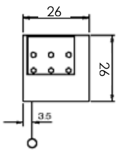
26x26 casing profile up to 7m base Power supply on the right
